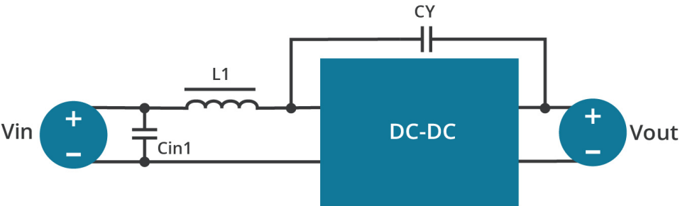
Figure 2 Single output
